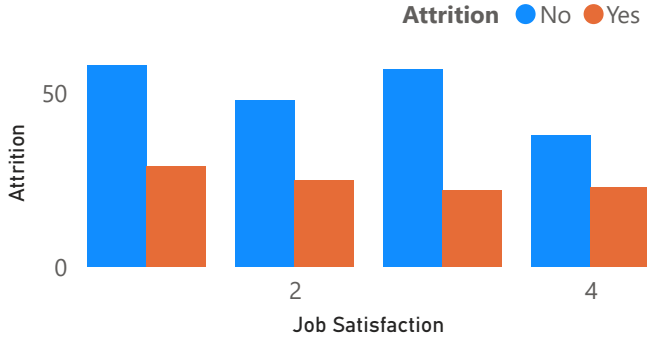
Attrition by Job Satisfaction
